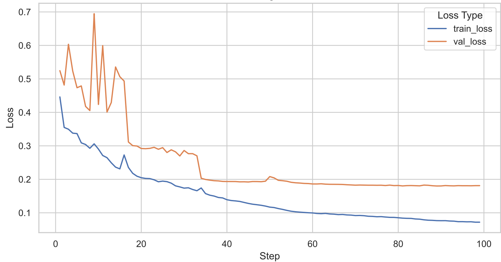
Learning Curve
